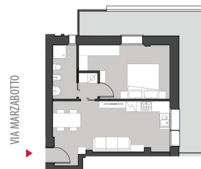
PIANO 1
